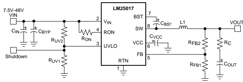
Reference Schematic for Selection of External Components
