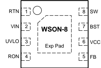
Figure 1. Top View (Connect Exposed Pad to RTN) Figure 2. Top View (Connect Exposed Pad to RTN)
