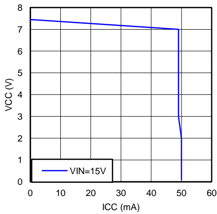
Figure 5. V_{CC} vs I_{CC}
