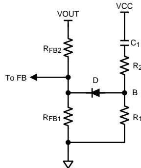
Figure 17. Soft-Start Circuit
