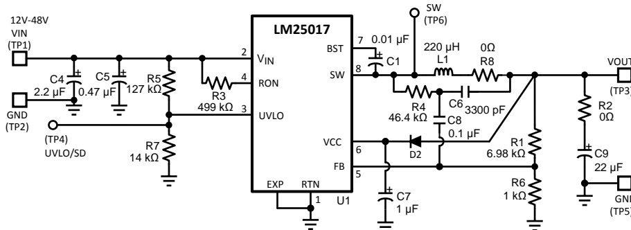
Figure 15. Final Schematic for 12 V to 48 V Input, and 10 V, 500 mA Output Buck Converter
